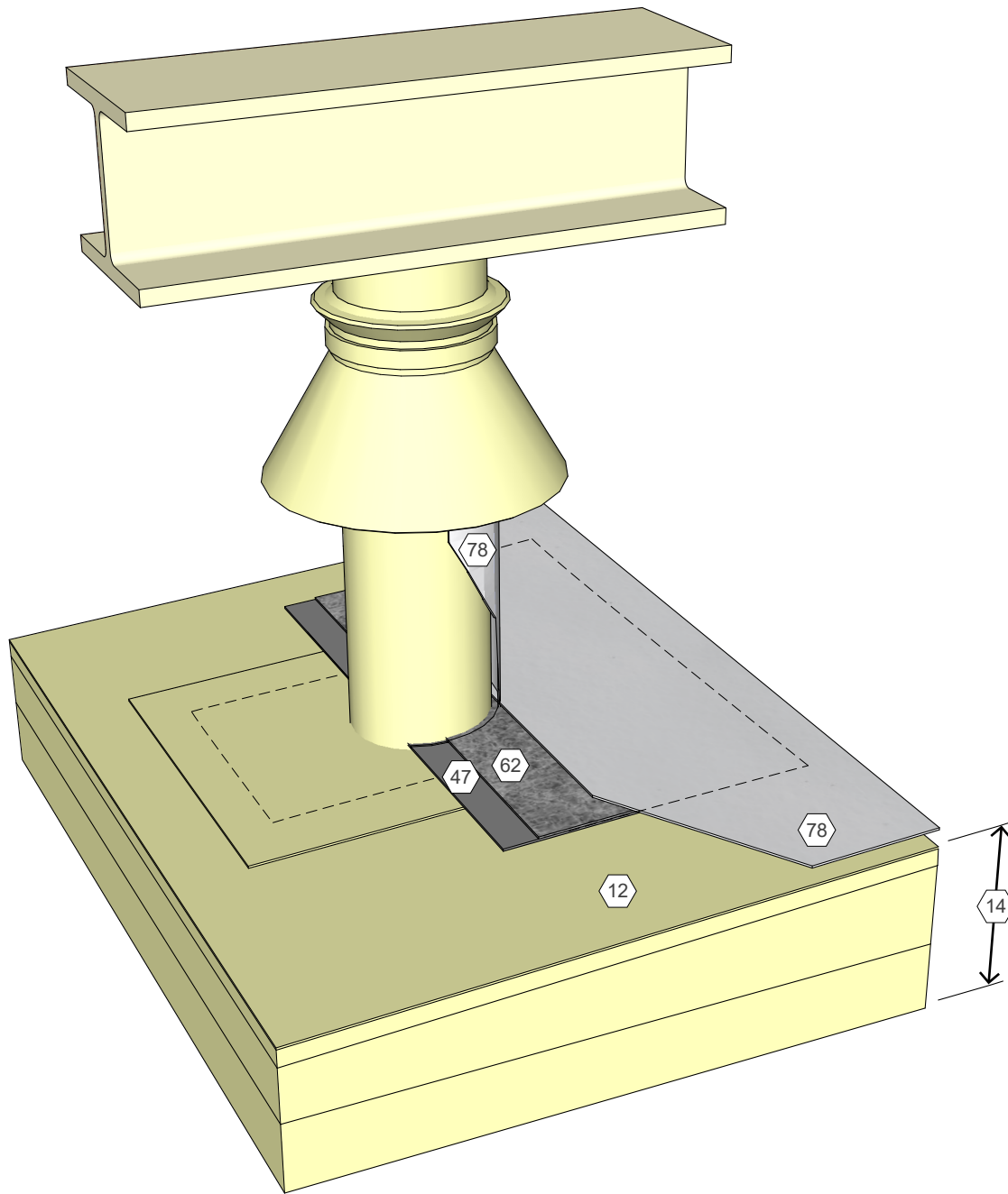
Alumanation 301 Restoration Detail, MB or Smooth BUR, Equipment Support Stand Leg Detail 19112
